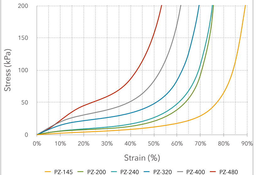
PZ series CFD Curve
